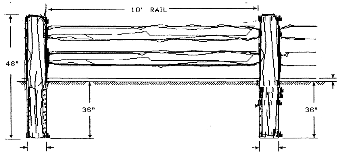
(ELEVATION VIEW)
